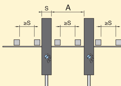
DISTANZA FRONTALE / FRONT DISTANCE
