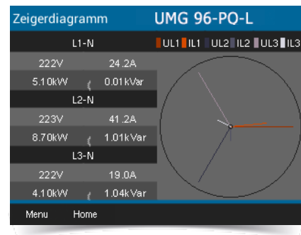
Fig.: Phasor diagram
