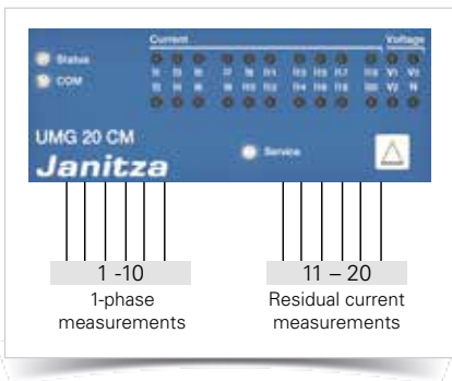
Fig.: 10 single-phase operational current measurements, 10 single-phase residual current measurements,
