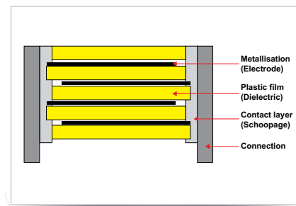
Fig.: Contacting (metal spraying) of the metallised Polypropylene film (Dielectric)
