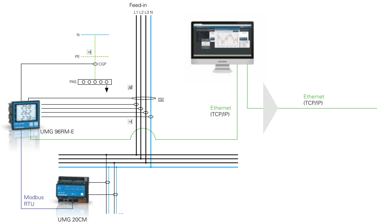
Fig.: The 20 channels of the UMG 20CM can be optionally used for residual current or operational current monitoring by utilising the corresponding current measurement transformer. In the case of residual current monitoring, the residual currents flowing to ground or any other path are acquired.
