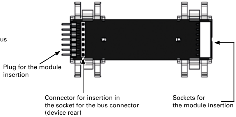
Bus connector for current measurement module
