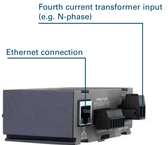
Fig.:UMG 96-PA with Ethernet connection
