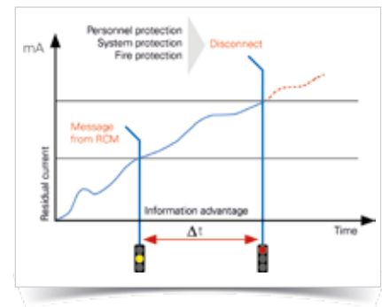
Fig. 1: Report prior to switching off - an aim of residual current monitoring (RCM)
