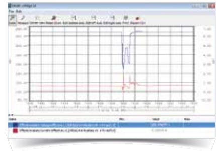
Fig.: Critical voltage dip with production standstill
