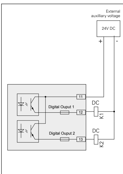
Fig. Example for two electronical relays connected to the digital outputs
