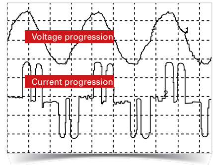
Fig.: Grid distortion effects through frequency converters
