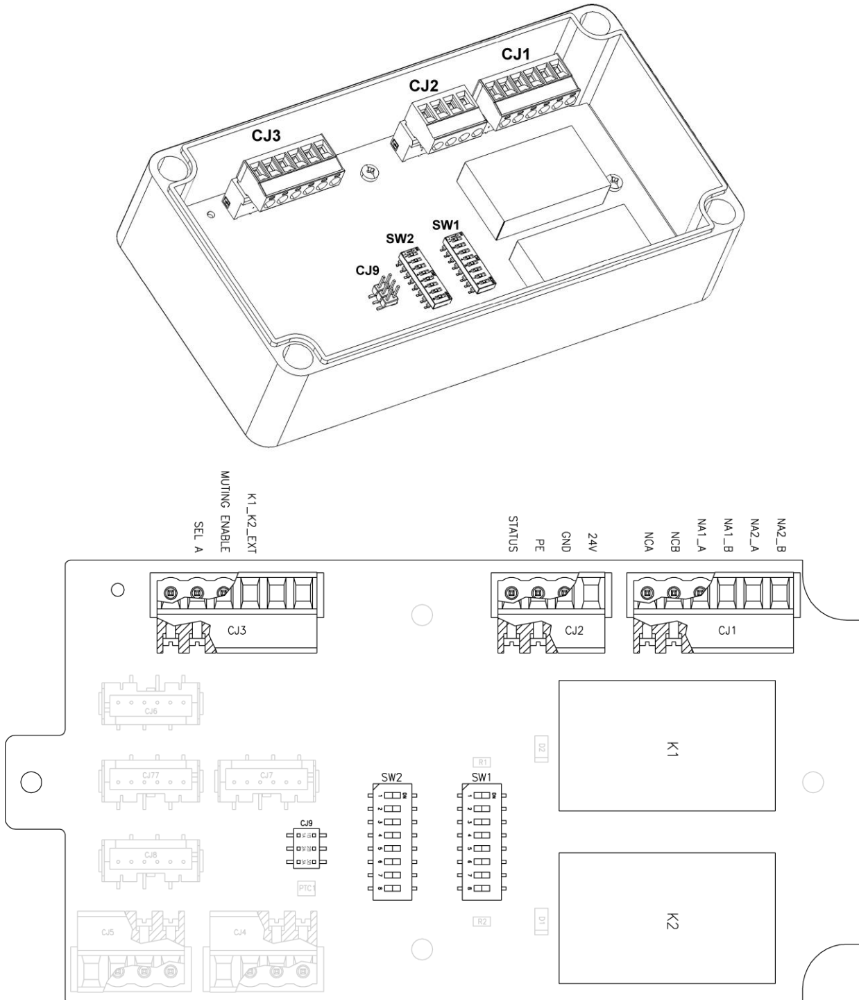
Figure 2 – Main board
