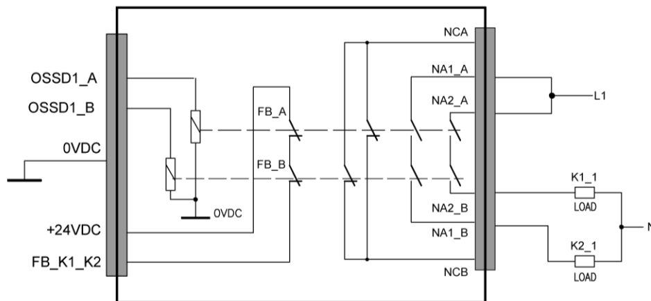
Figure 3 – M SGO BOX connection sample
