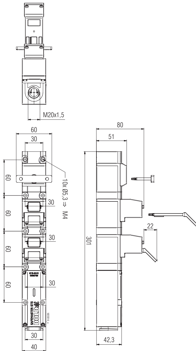
RX11BM/K Clearance tolerances ± 2%
