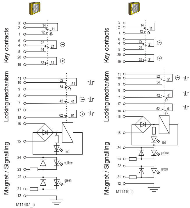
Fig. 1: Solenoid locking activated: Magnet locked, 1st key removed, 2nd key inserted
