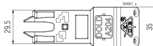
Steckschlüssel
