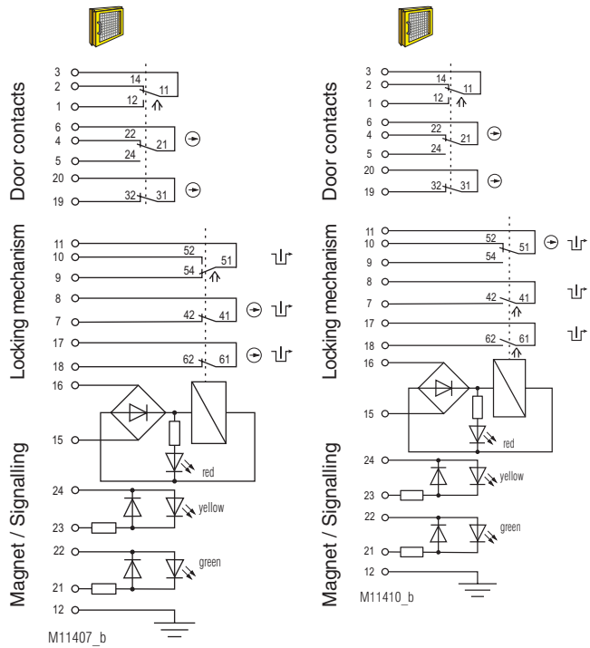
Fig. 1: Guard locking in activated state: solenoid interlocked, key inserted
